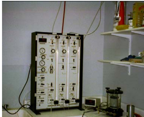
Photos (top to bottom): Drilling rig at Gardner Denver; Flexible wall permeability test panel; Nuclear moisture/density testing.
